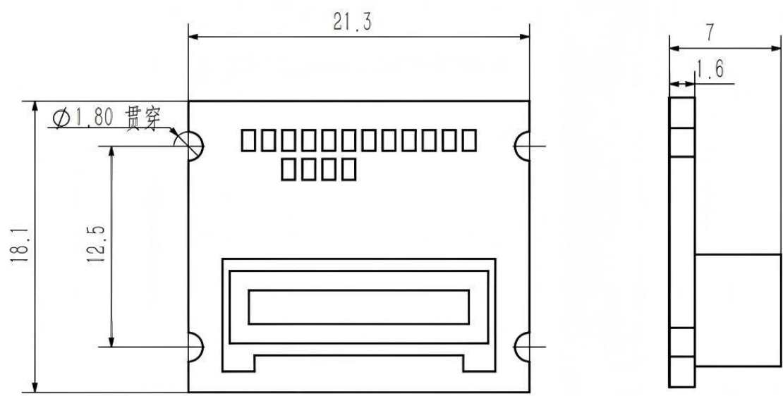
Dimension Drawing
