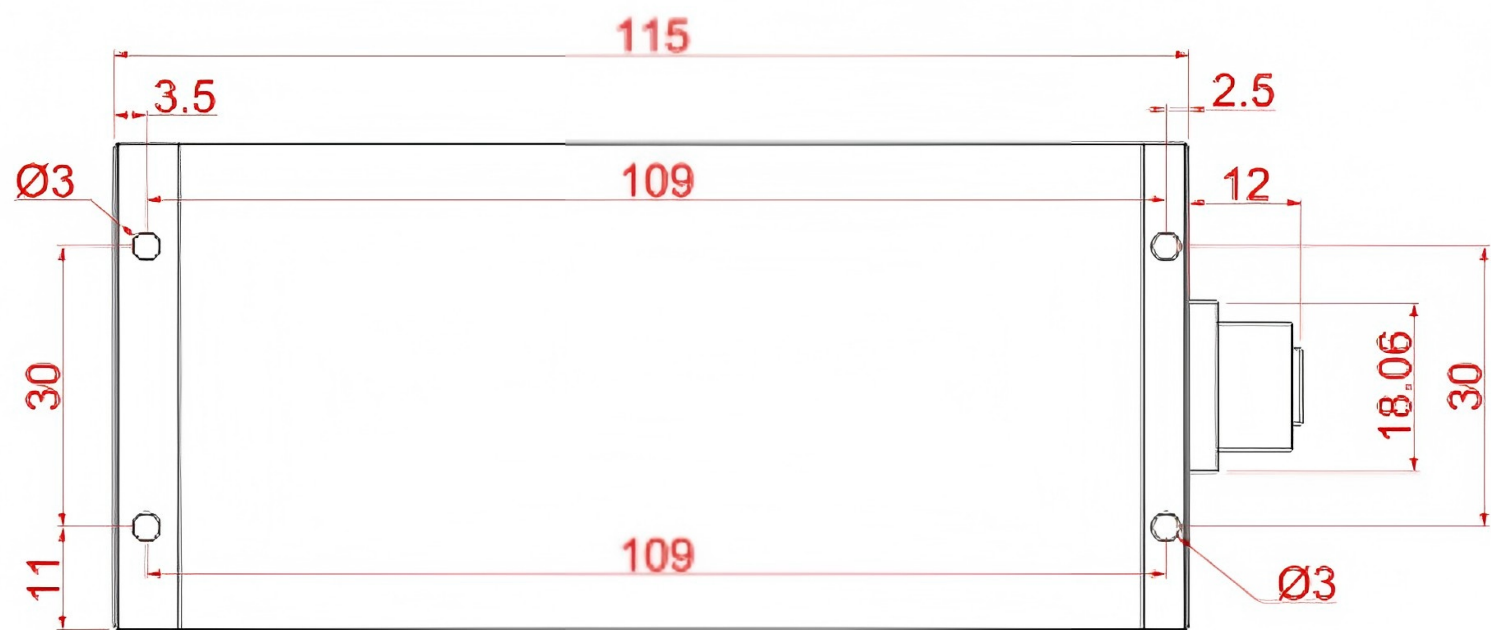
Bottom View
