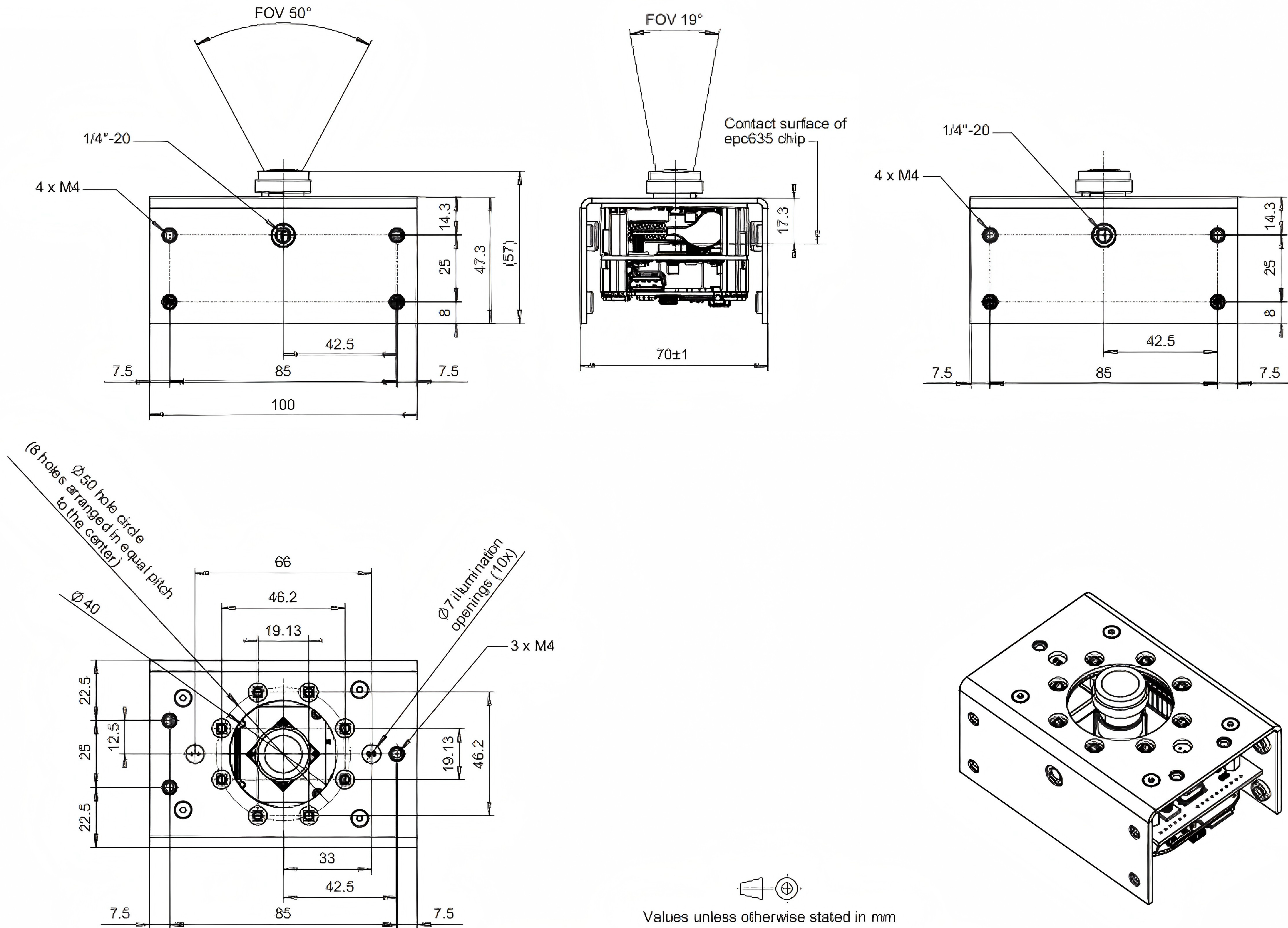
Figure 9: Reference dimensions of the optical axis and illumination
