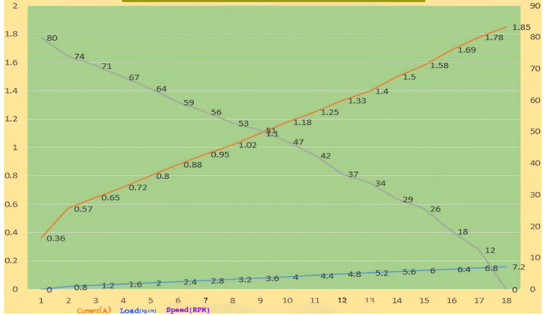
ST-3009-C001-Brushless Motor Performance Curve Graph-6V
