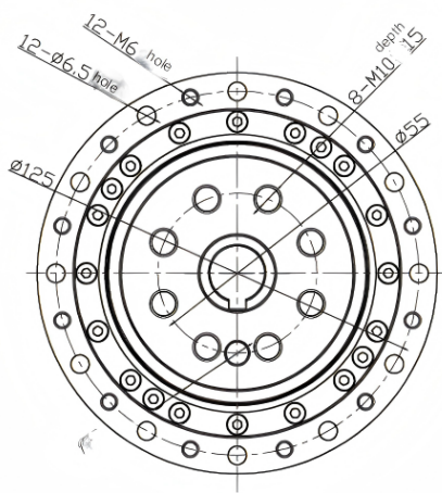
Output shaft end
