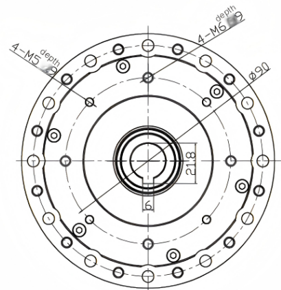
Input shaft end
