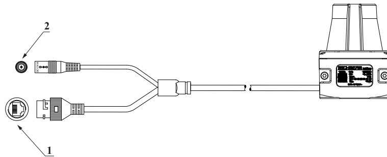
Figure 5.1: LiDAR Cable Diagram
