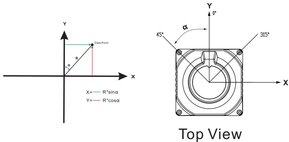
Figure 8.3: LiDAR Polar Coordinate and X, Y, Z Coordinate Mapping
