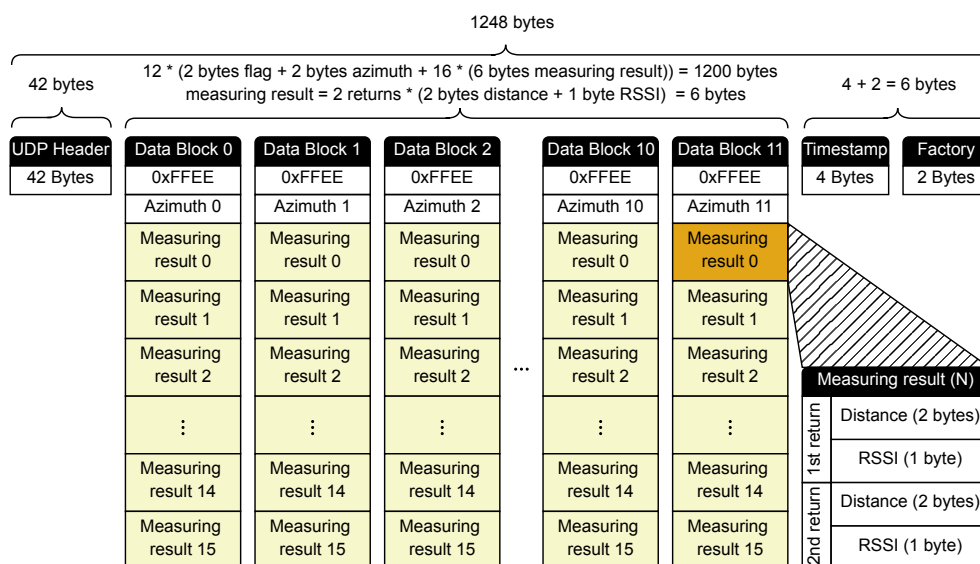
Figure 7.1: MSOP Packet Structure
