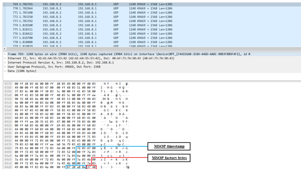
Figure 7.4: MSOP Packet Demonstration Data 2
