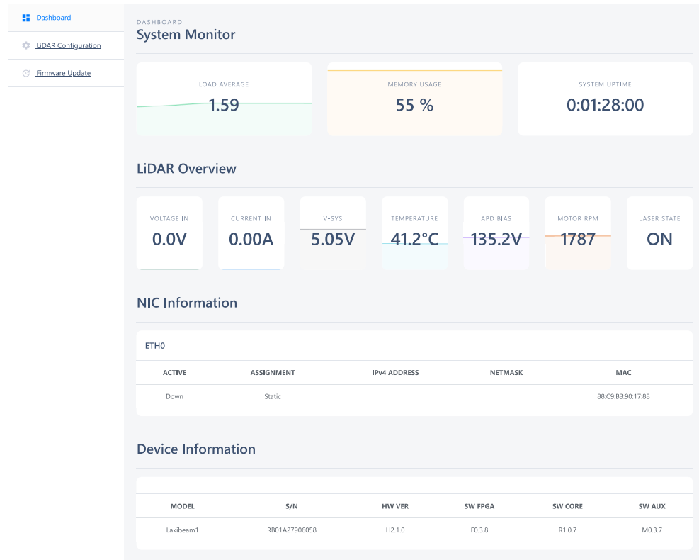
Figure 6.1: Dashboard Page
