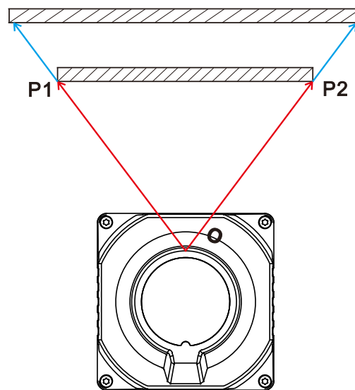
Figure 6.7: Principle of LiDAR Veiling Effect
