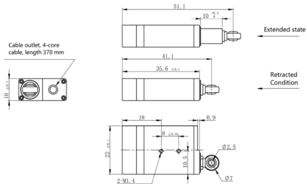
DH08Z-10-01-1-RS Outline Drawing
