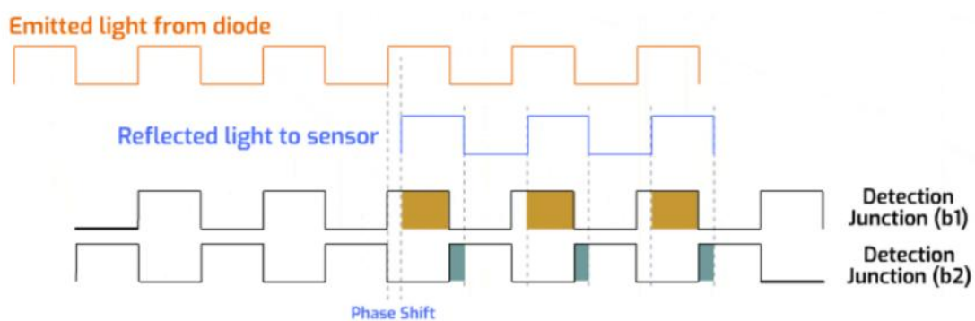
Figure 2.1 Detection schematic
