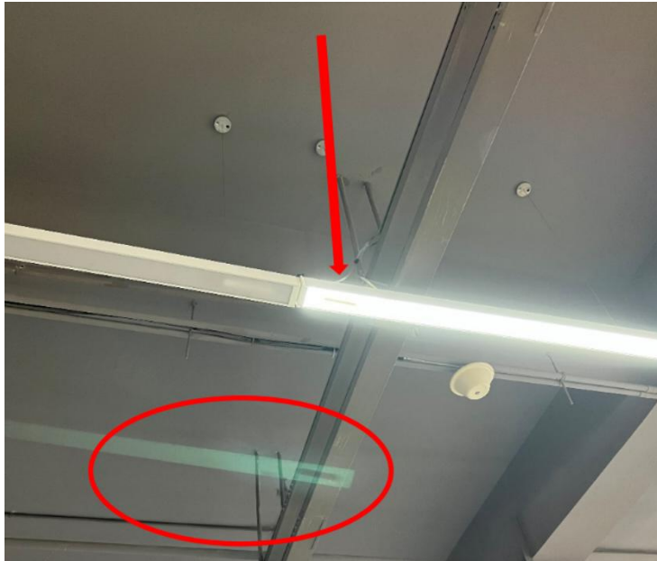
Figure 3.15 Stray light affects ghost and flare
