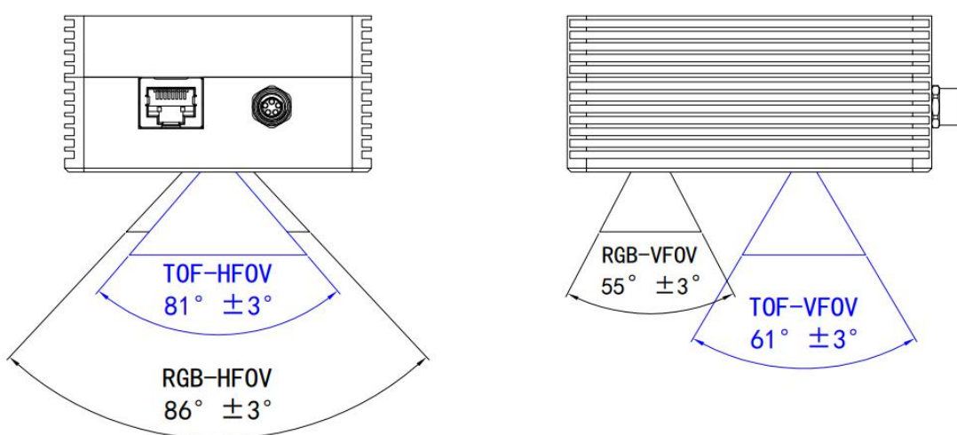
Fig. 3.7 Field of view of M4Pro 850
