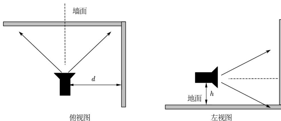
Figure 3.13 Installation Method 3
