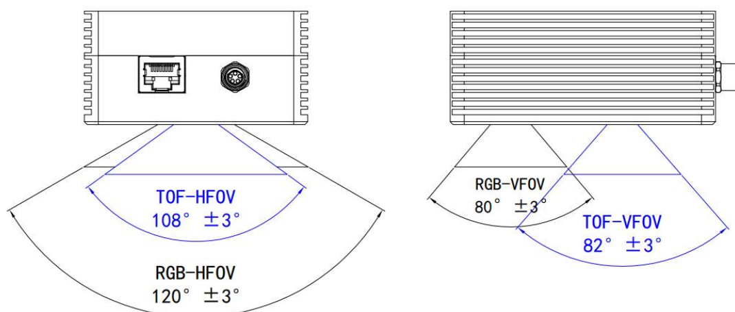
Fig. 3.6 Field of view of M4Pro Wfov
