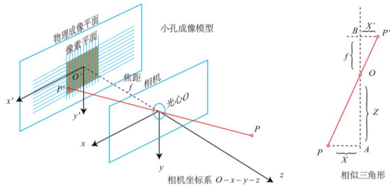
Figure 3.9 Optical coordinate system
