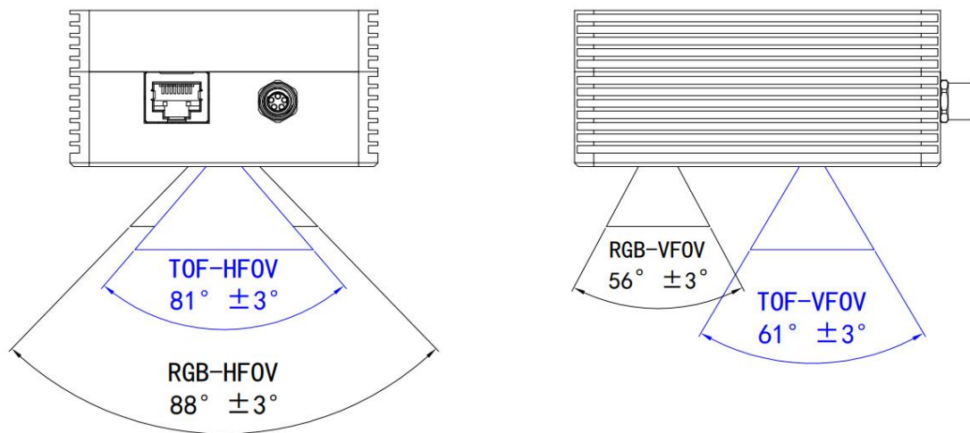
Figure 3.5 M4Pro field of view range
