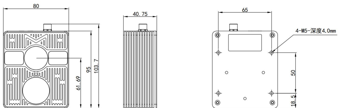
Figure 3.8 M4Pro camera size chart
