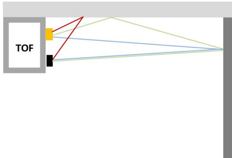
Figure 4.2 Camera installation diagram
