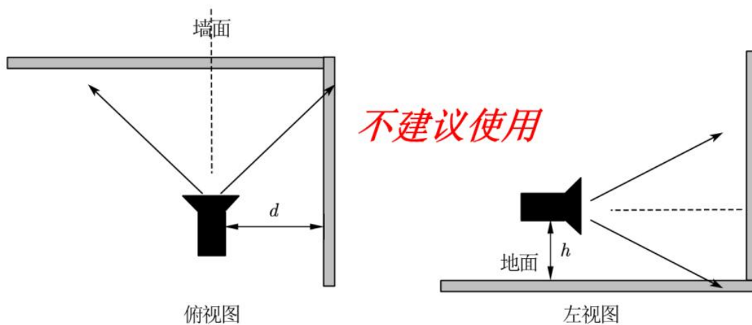
Figure 3.16 Unrecommended Installation Methods
