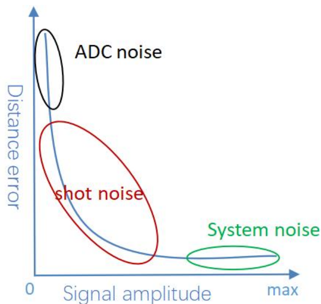
Figure 4.3 Relationship between measurement accuracy and signal strength
