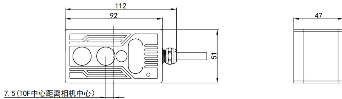
Figure 3.5 M4 Mega camera size chart
