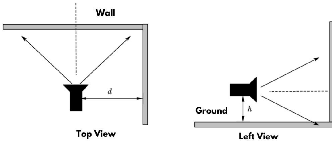
Figure 3.10 Installation Method 3
