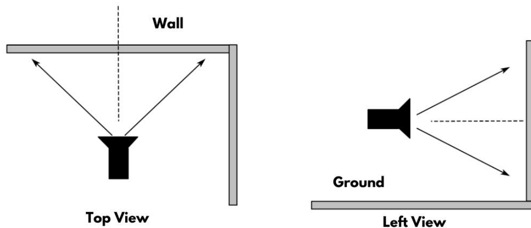
Figure 3.8 Installation Method 1
