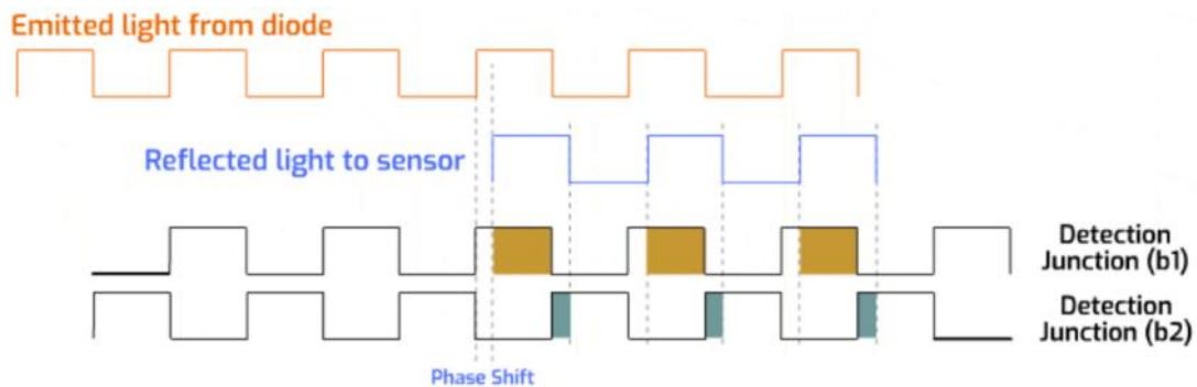
Figure 2.1 Detection schematic
