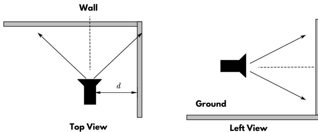
Figure 3.9 Installation Method 2
