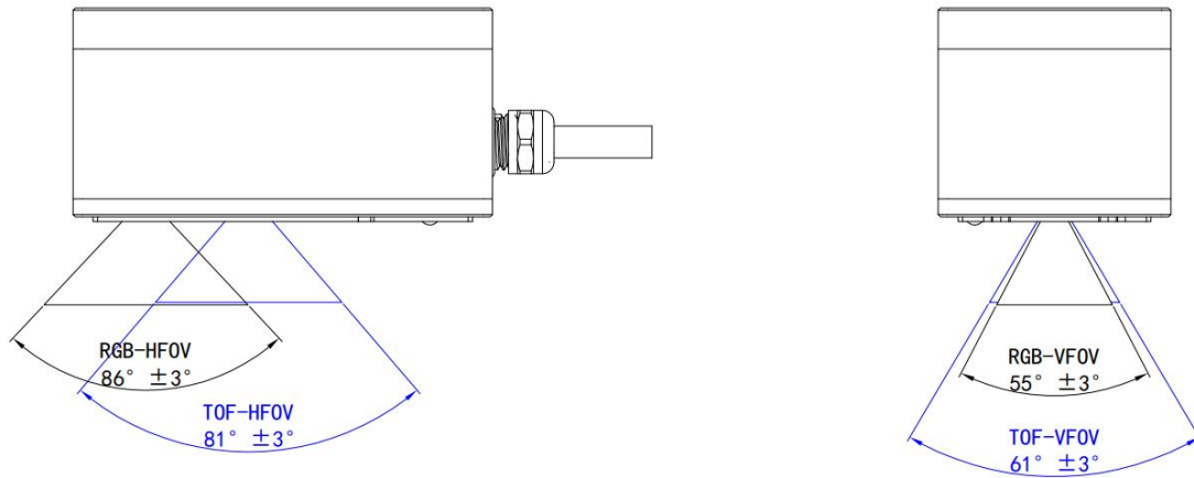
Figure 3.4 Field of view range
