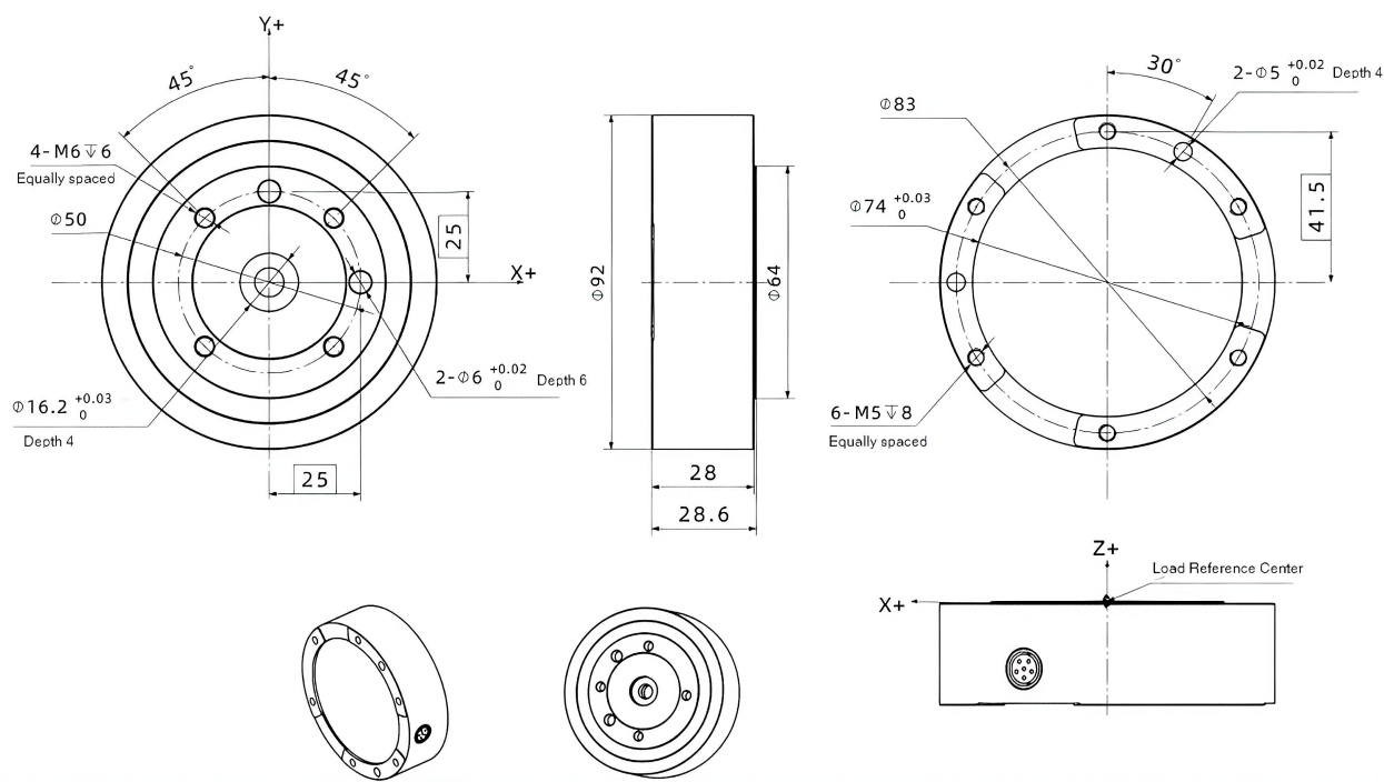
Product Installation Dimensional Drawing
