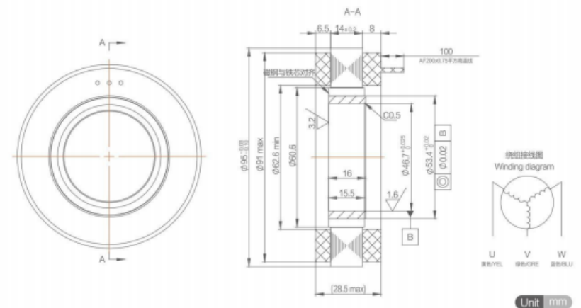
Frameless torque motor
