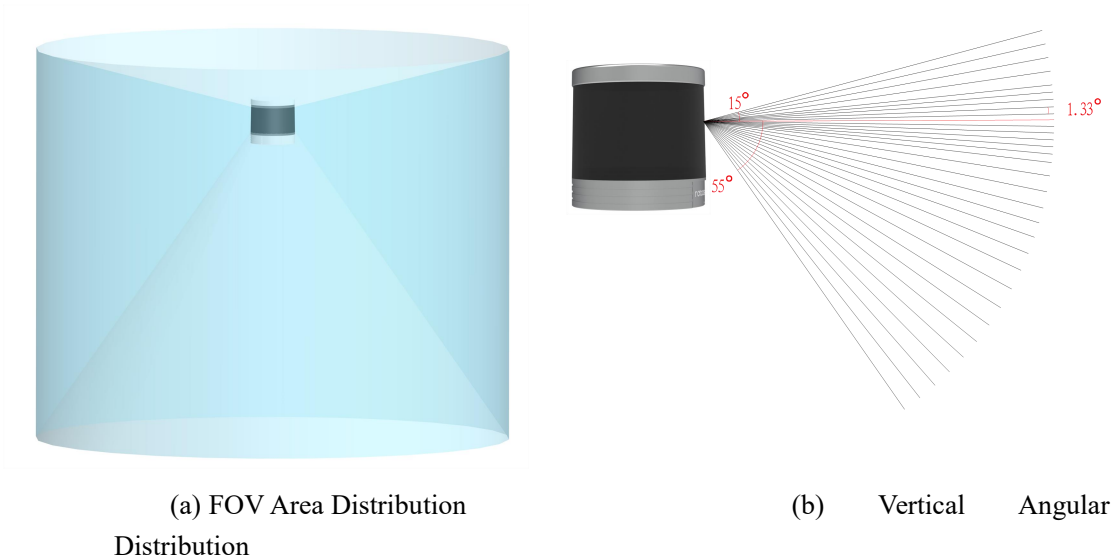
Figure 2 70° FOV Illustration
