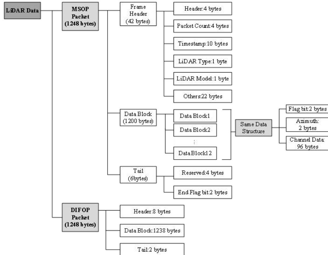
Figure 16 LiDAR Data Structure Illustration
