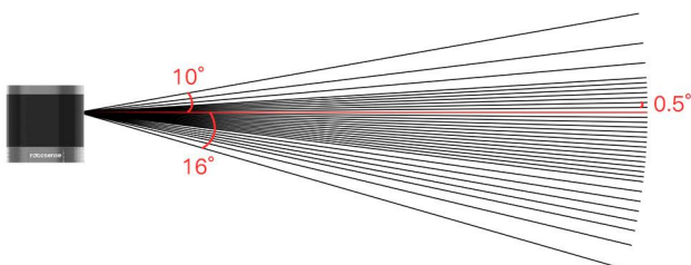
Helios 32: 26^\circ Vertical FOV, gets denser in the middle part, up to 0.5^\circ vertical angular resolution
