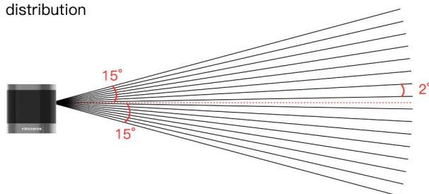
Helios 16: 30^\circ Vertical FOV, 16-Beam even distribution
