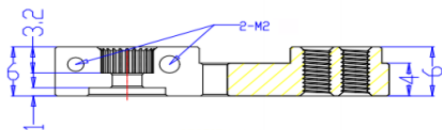
SECTION X-X
